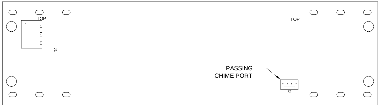
REAR VIEW
